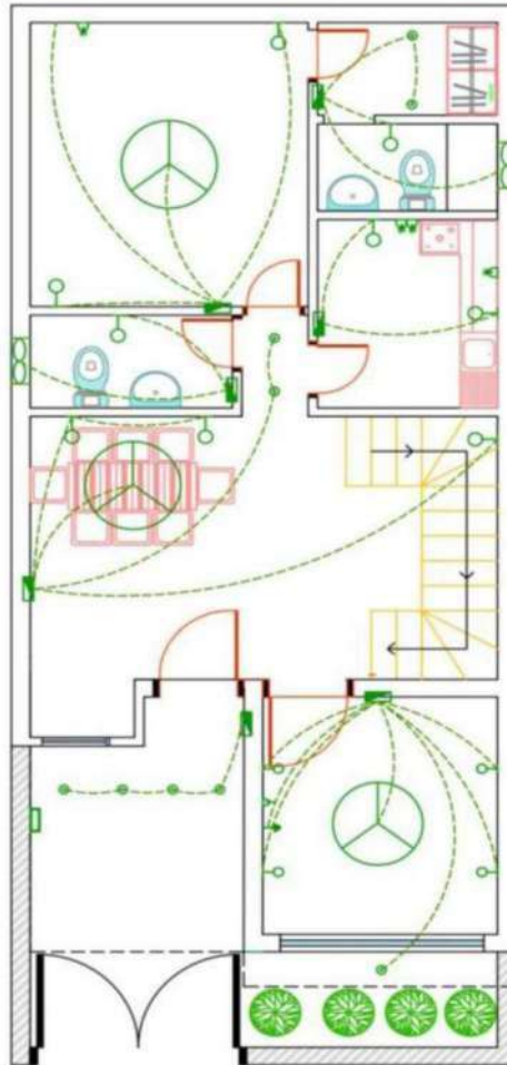
FIRST FLOOR ELECTRICAL
