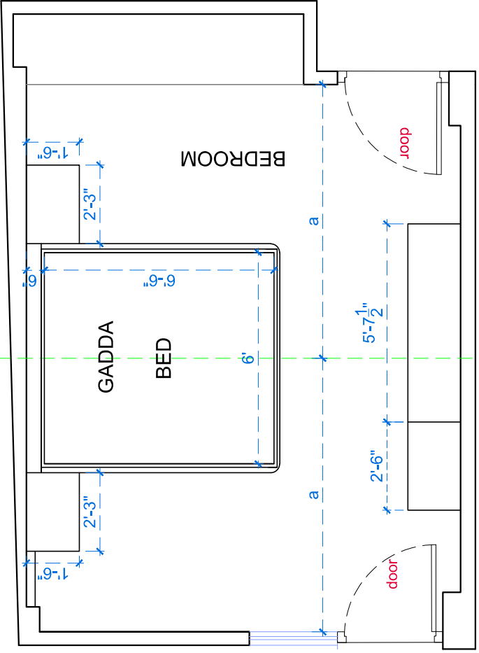
PLAN
