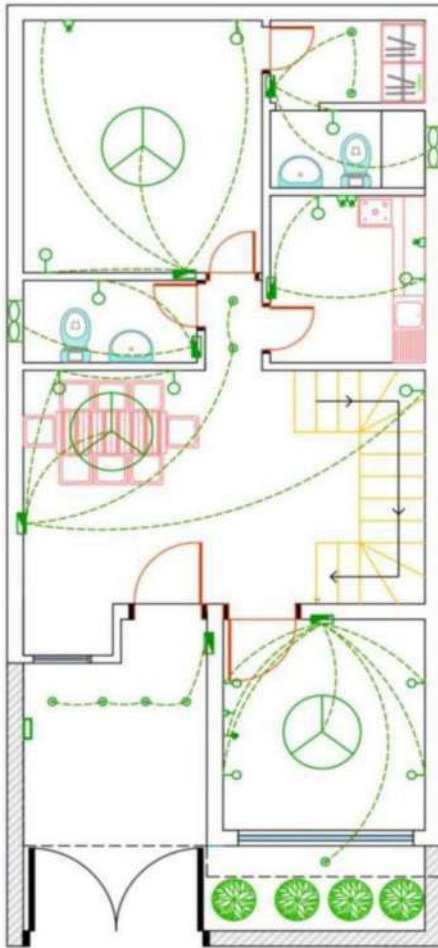
GROUND FLOOR ELECTRICAL
